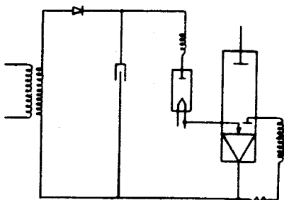
ELEMENTARY CIRCUIT FOR CAPACITOR FIRING
