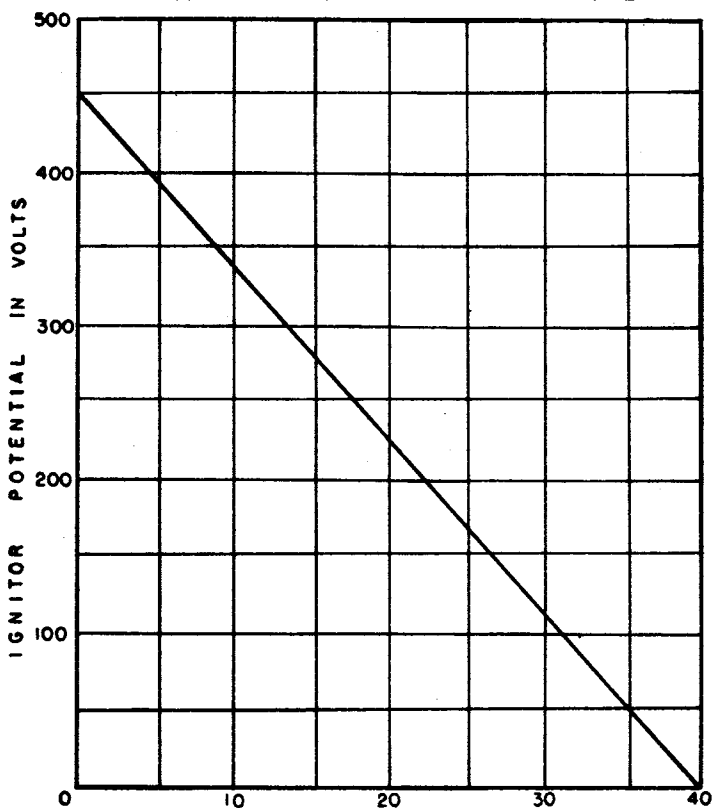
MINIMUM VOLT-AMPERE REQUIREMENTS FOR SEPARATE-EXCITATION FIRING SYSTEMS
