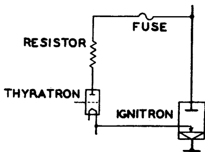
ELEMENTARY CIRCUIT FOR ANODE FIRING
